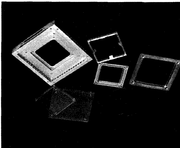
Figure 6. Expanded view of test fixture.
