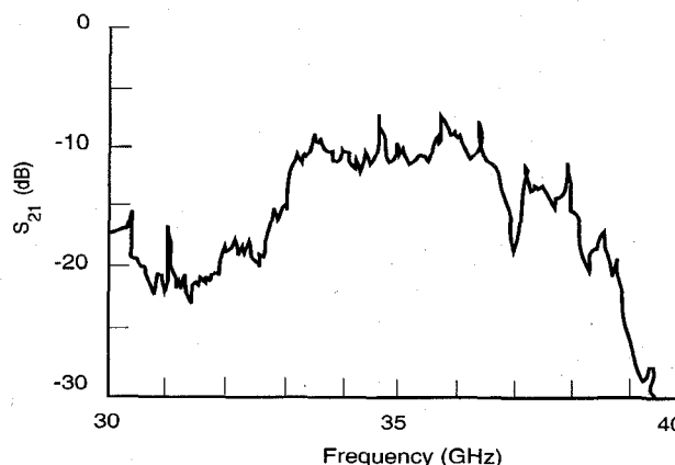
Figure 8. Measured response of passive array.
