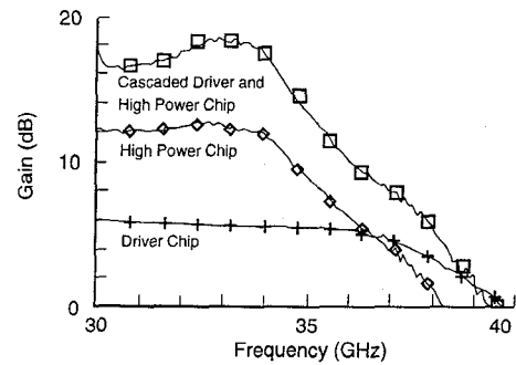
Figure 5 Cascaded small-signal gain of MMIC chips.
