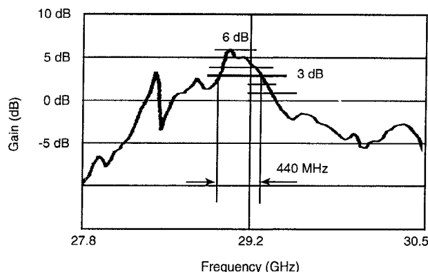
Figure 9. Small-signal gain of amplifier array.
