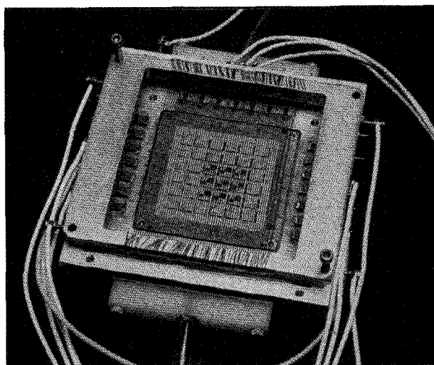
Figure 1. 6x6 hybrid amplifier array.
