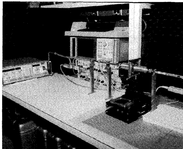
Figure 7. Small-signal quasi-optical test setup.
